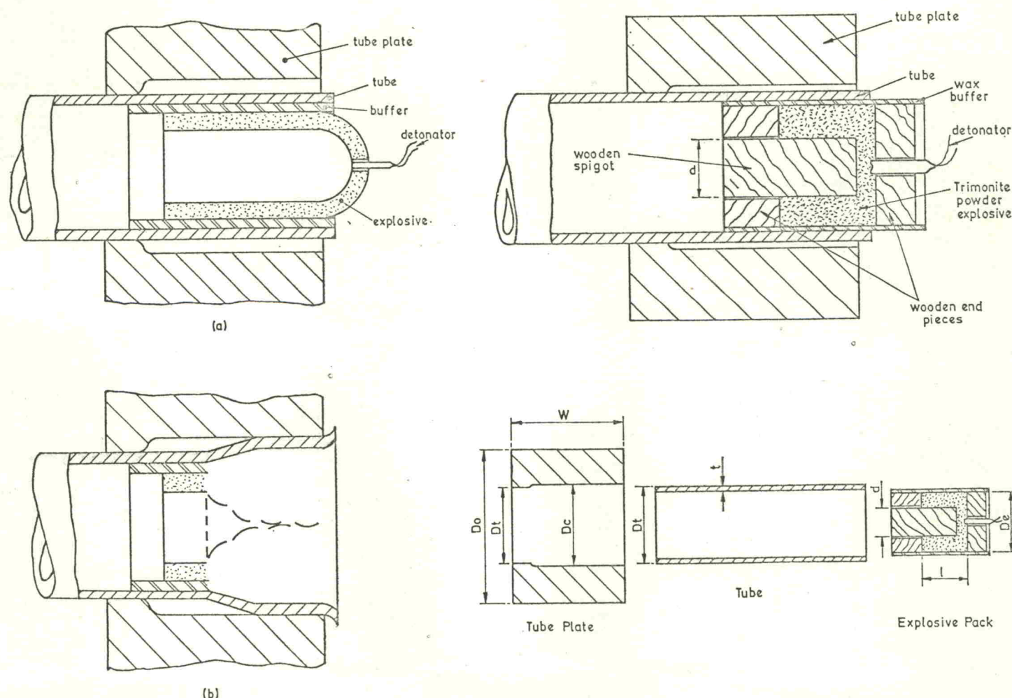
38 Welding of tubes to tube plates using a low-detonation-velocity explosive. (a) Before detonation; (b) after detonation.
